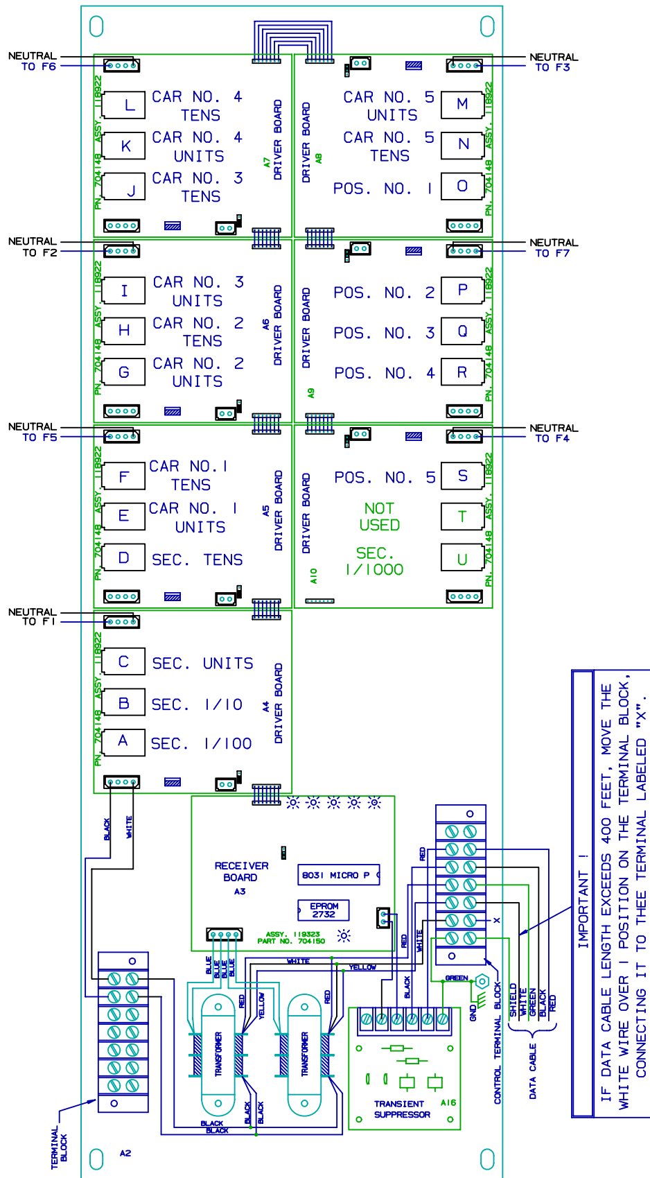
CONTROLLER ASSEMBLY
