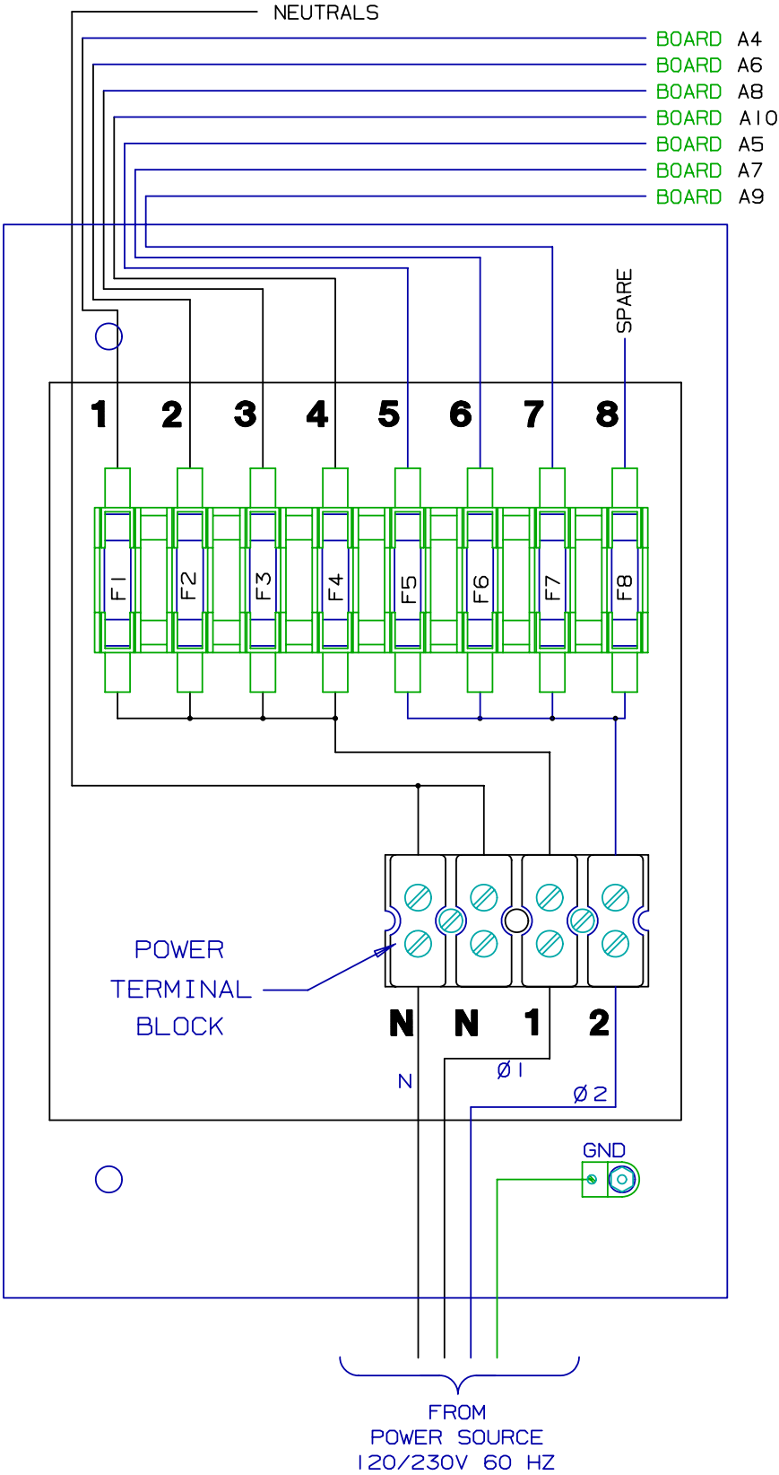
POWER WIRING
