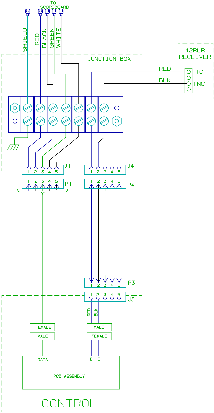
SINGLE JUNCTION BOX WIRING
