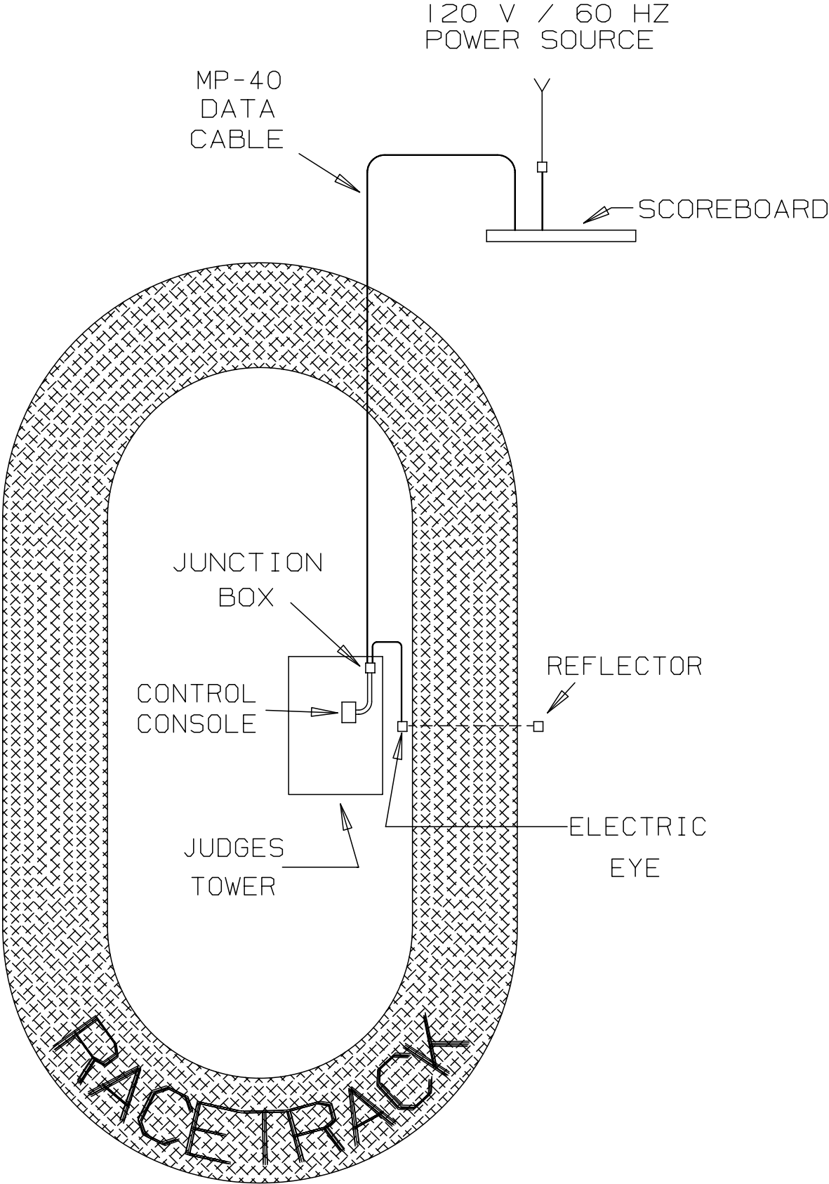
SYSTEM LAYOUT
